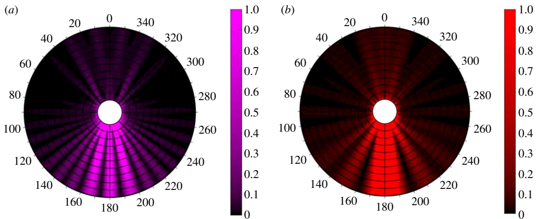
Figure 1. Modelled scattered light intensity for a 2\ \mu\text{m} diameter single cylinder, n = 1.536 , at wavelengths of 350\ \text{nm} (a) and 633\ \text{nm} (b). The diameter of the modelled region is 14\ \mu\text{m} . The angle in degrees is annotated at the edge of the circular region. Zero degrees corresponds to centre of the backscattered light and 180^\circ to the centre of the forward-scattered light. The computation for 2\ \mu\text{m} was truncated at 30 cylindrical harmonic modes and that for 6\ \mu\text{m} to 80 modes. The intensity map is an average of scattered light polarized parallel and perpendicular to the cylinder axis. The intensity scale is normalized to that of the incident wave and the colour scale allows lower level intensities values to be visualized.
